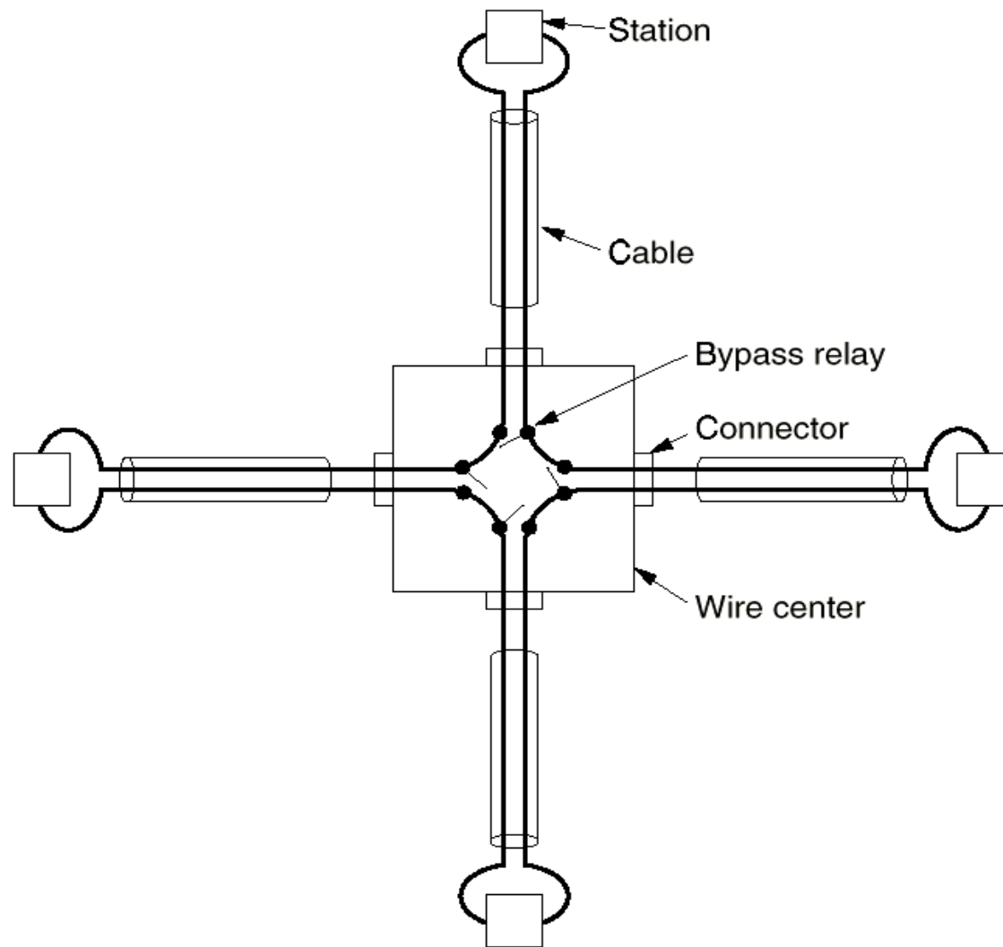
Fig. 4-29. Four stations connected via a wire center.
