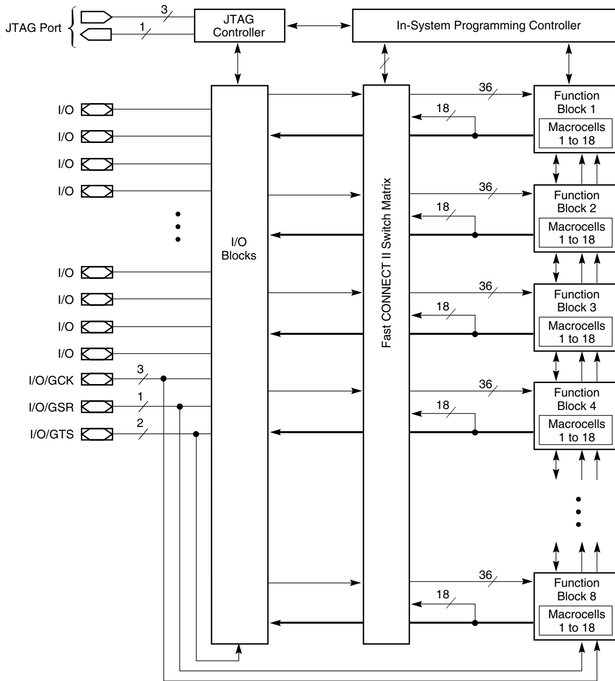
Figure 2: XC95144 Architecture
