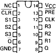
SN54L71 ... J PACKAGE (TOP VIEW)
