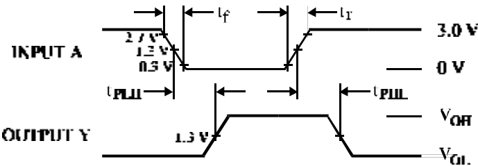
Figure 1. Switching Waveforms
